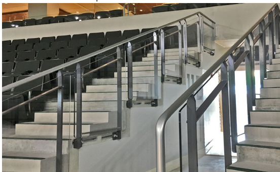
Lexan Rail features transparent plastic panels and rectangular posts.
