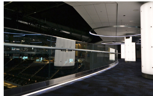
Track Rail top mounted to a rolled steel angle and outfitted with LED lighting.
