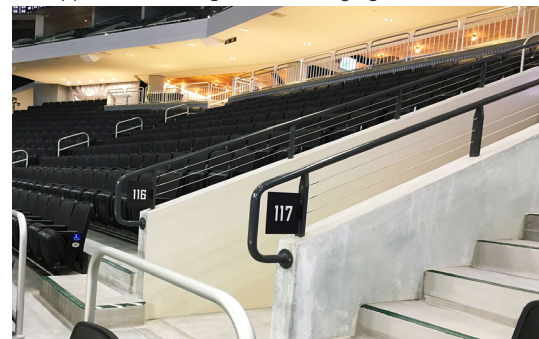
Liquid painted steel railing with cable infill brings sleek style to the arena.
